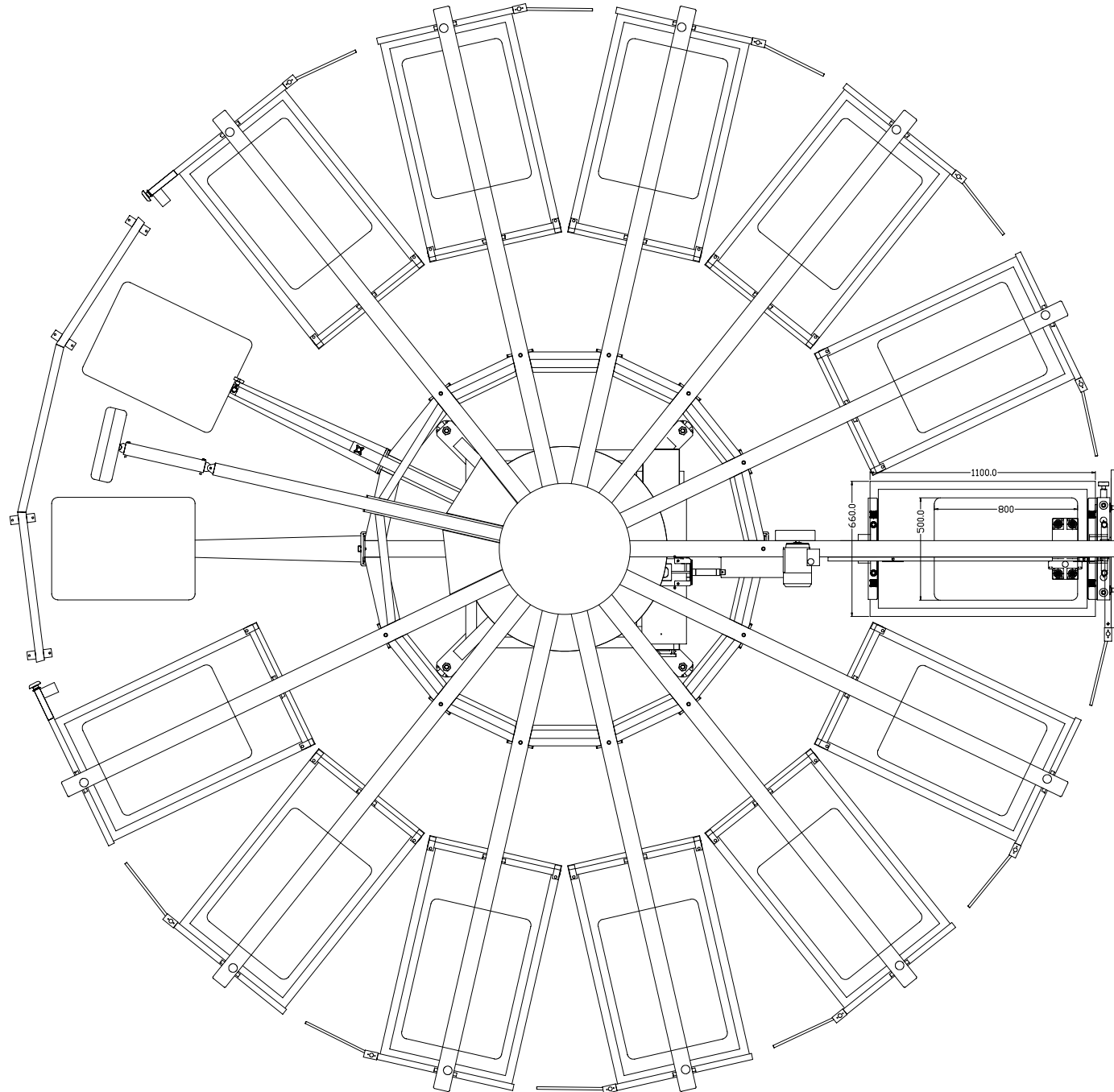
PRISM I 14s 12c 50 x 70 cm print area configuration
